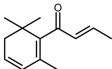
2-Buten-1-one, 1-(2,6,6-trimethyl-1,3-cyclohexadien-1-yl)-
